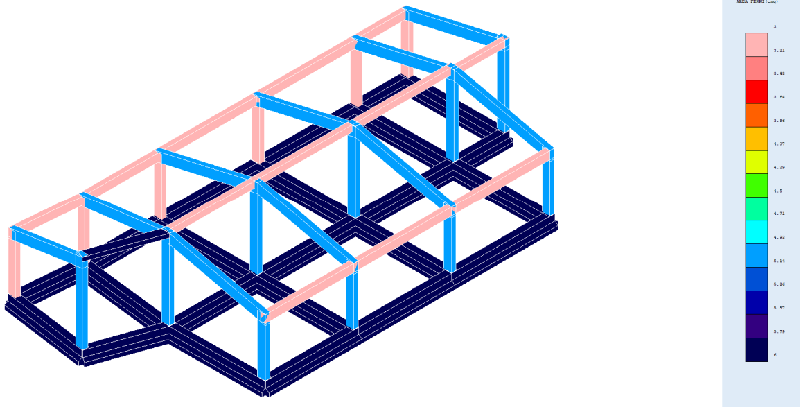
Fig. 54 – Area ferri (cmq)
